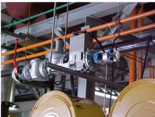
Typical GTI Bi-Fuel Gas Train Mounting Options: “Trapeze” Method (left), and “Bottom” Method (right)
