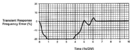
Typical Responses to 100% Block Load Application
