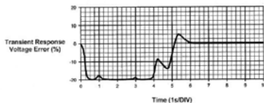
Bi-Fuel Operation (70% Gas)
