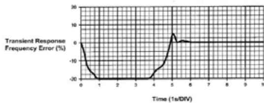
Typical Responses to 100% Block Load Application
